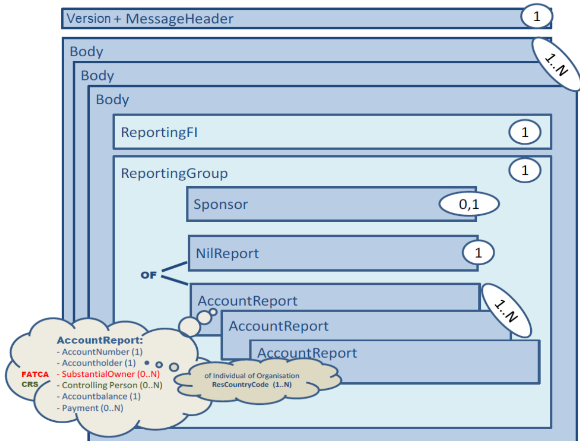
Figure 1b: Cardinality within the FATCA CRS XML message schema 2.2
