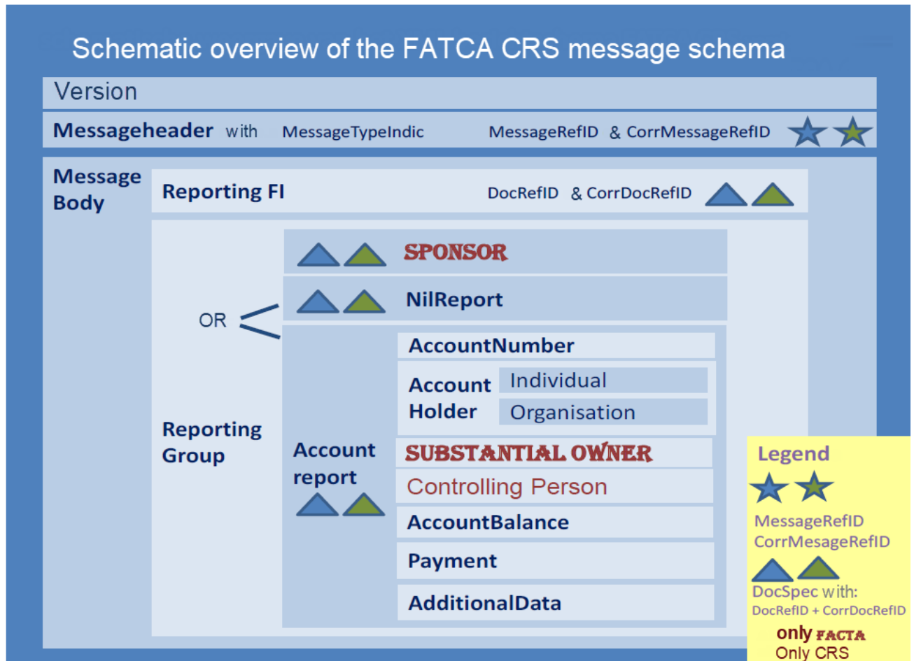
Figure 1a: Schematic overview of the FATCA CRS XML message schema 2.2
